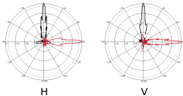
RF Antenna Patterns
